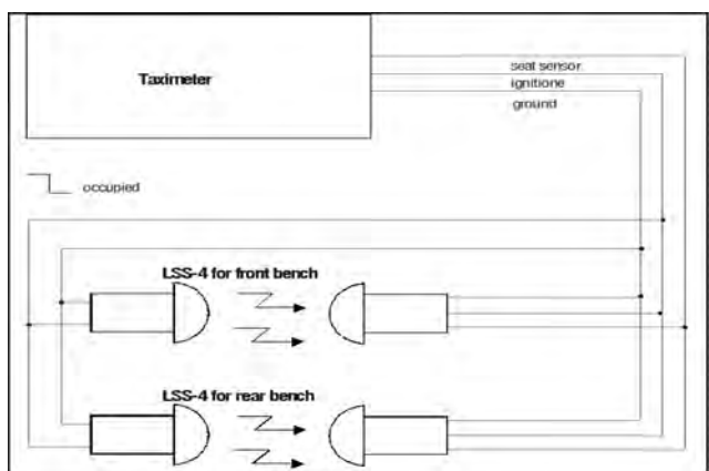
Solution with taximeter from other manufacturer
