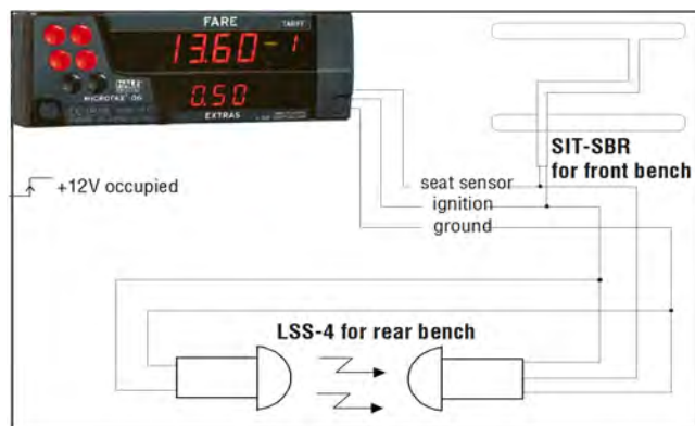
Combination SIT-SBR and LSS-4
